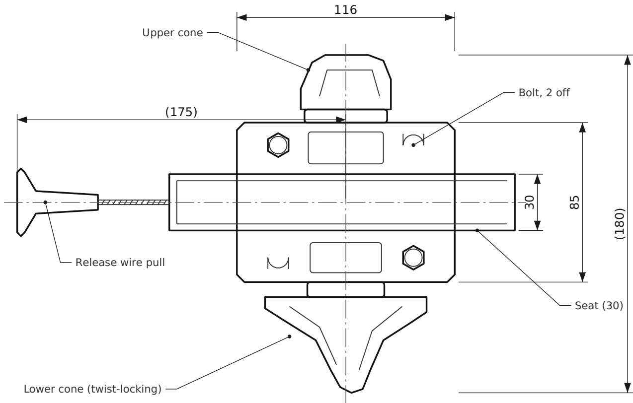
FRONT ELEVATION Scale 1:2 · locked position
