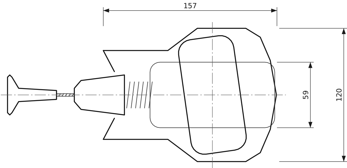
PLAN Scale 1:2 · viewed from above
